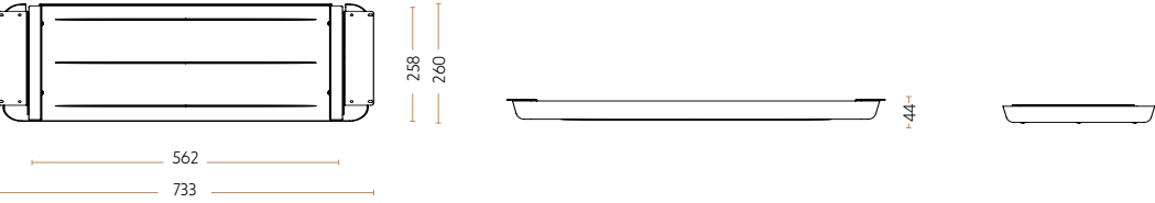
Filt skuffe - large 6000-0083
