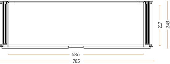
Bambusskuffe large 4090-C
