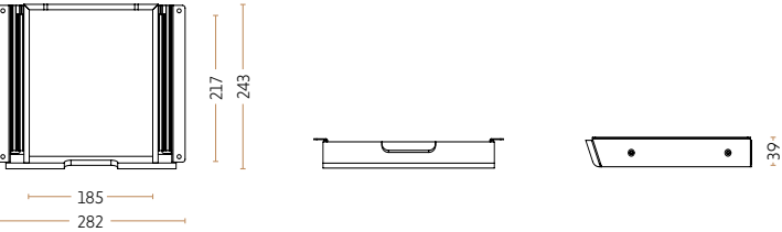
Bambusskuffe large 4090-C
