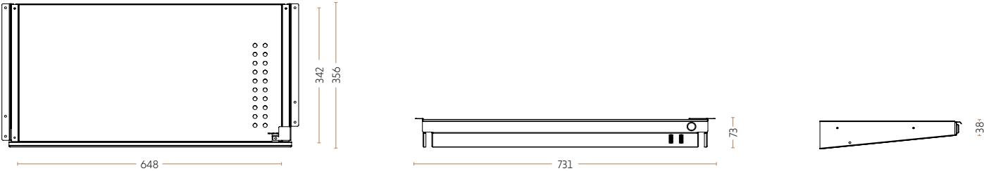
Laptop tray 2014 with lock 4070-9005-L // 4070-9006-L // 4070-9016-L
