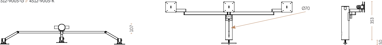
Future Flex for three monitors 4512-9005-G // 4512-9005-K
