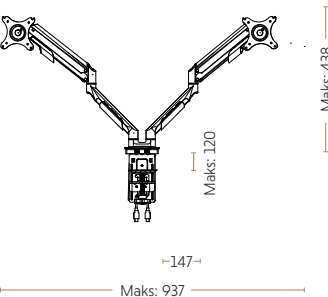
Monitorarm for two monitors 4402-9005
