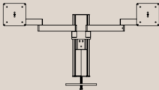
Monitor pole for two monitors. Available in two versions Monitor pole: 300 mm. // Extension arms: 2 x 334 mm. Find more information on page 68-69
