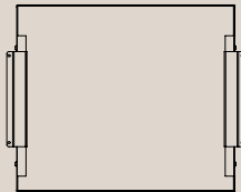
Horizontal laptop holder - large H: 106 mm. // W: 526 mm. // D: 411 mm. Find more information on page 60-61
