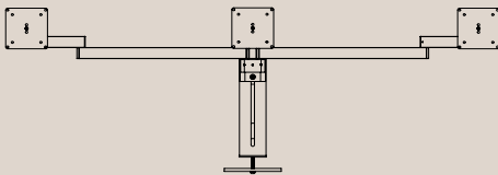
Future Flex for three monitors. Available in two versions Monitor pole: 350 mm. // Extension arms: 2 x 597 mm. + 1 x 37 mm. Find more information on page 64-65
