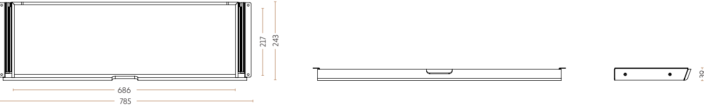
Bamboo pen tray - large 4090-C // 4090-S // 4090-CI (bamboo insert included) // 4090-SI (bamboo insert included)
