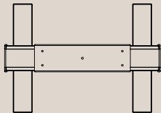
Horizontal CPU-holder H: 30-90 mm. // W: 260-460 mm. // D: 340 mm. Find more information on page 52-53
