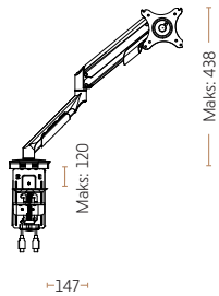
Monitorarm for one monitor 4401-9005
