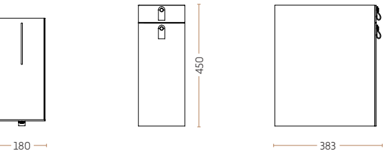
Mobile cassette with two drawers 2020-0700-9005 // 2020-0700-9016
