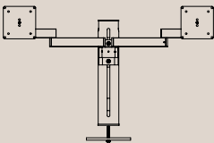
Future Flex for two monitors. Available in two versions Monitor pole: 350 mm. // Extension arms: 2 x 334 mm. Find more information on page 64-65
