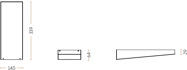
Insert for Laptop tray 2014 4070-9005-TR
