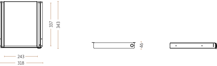
Lockable tablet tray - narrowed model, with rubber drawer liner and lock 4010-9005-LT // 4011-9006-LT // 4012-9016-LT
