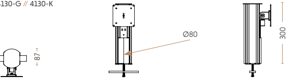
Monitor Pole for one monitor 4130-G // 4130-K
