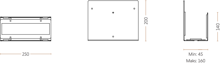
Wall mounted CPU-holder 1560-9005 // 1590-9006
