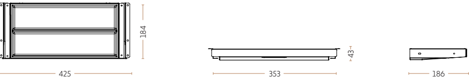
Ultra Pen - small, with removable plastic insert 4042-9005 // 4043-9006 // 4045-9016
