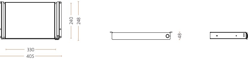
Lockable tablet tray - widen model, with rubber drawer liner and lock 4015-9005-LT // 4016-9006-LT // 4017-9016-LT
