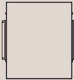
Horizontal laptop holder - extra small H: 106 mm. // W: 396 mm. // D: 411 mm. Find more information on page 60-61
