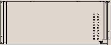
Laptop tray 2014 with lock H: 38 mm. // W: 731 mm. // D: 356 mm. Find more information on page 42-43
