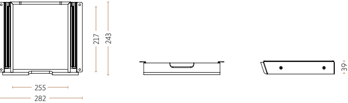
Bamboo pen tray - large 4090-C // 4090-S // 4090-CI (bamboo insert included) // 4090-SI (bamboo insert included)
